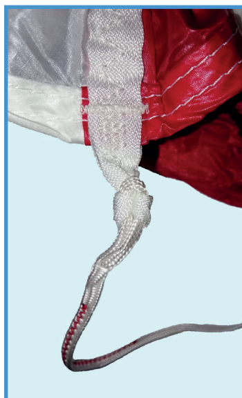
Liaison coupole et suspente - Suspente nylon/ galon nylon
